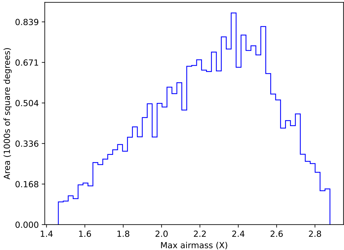
too_elab_r32_d3_griz_v3.4_10yrs All sky y band: Max airmass
