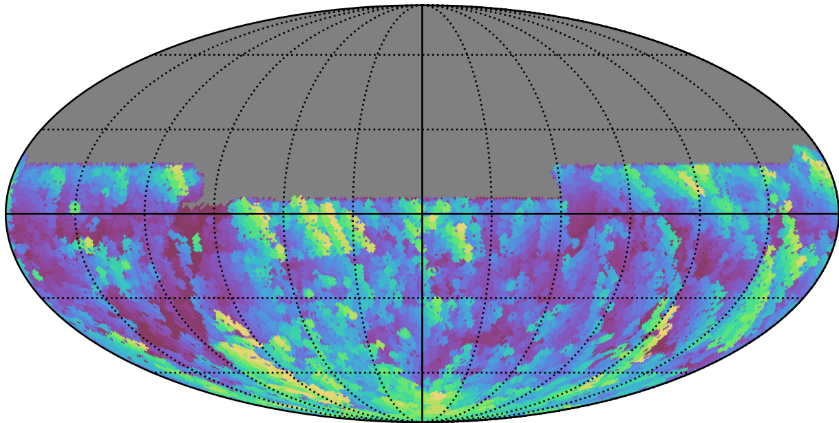
too_elab_r32_d3_griz_v3.4_10yrs All sky u band: Max airmass
