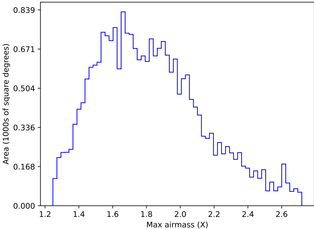
too_elab_r32_d3_griz_v3.4_10yrs All sky u band: Max airmass
