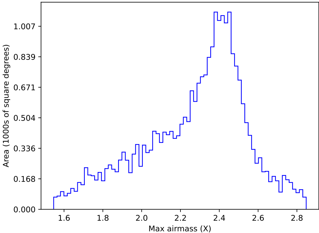
too_elab_r32_d3_griz_v3.4_10yrs All sky r band: Max airmass
