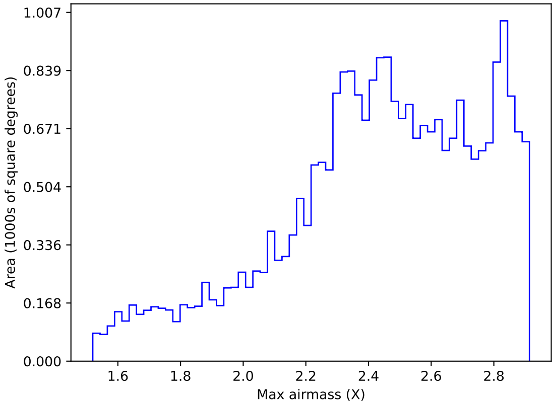
too_elab_r32_d3_griz_v3.4_10yrs All sky i band: Max airmass
