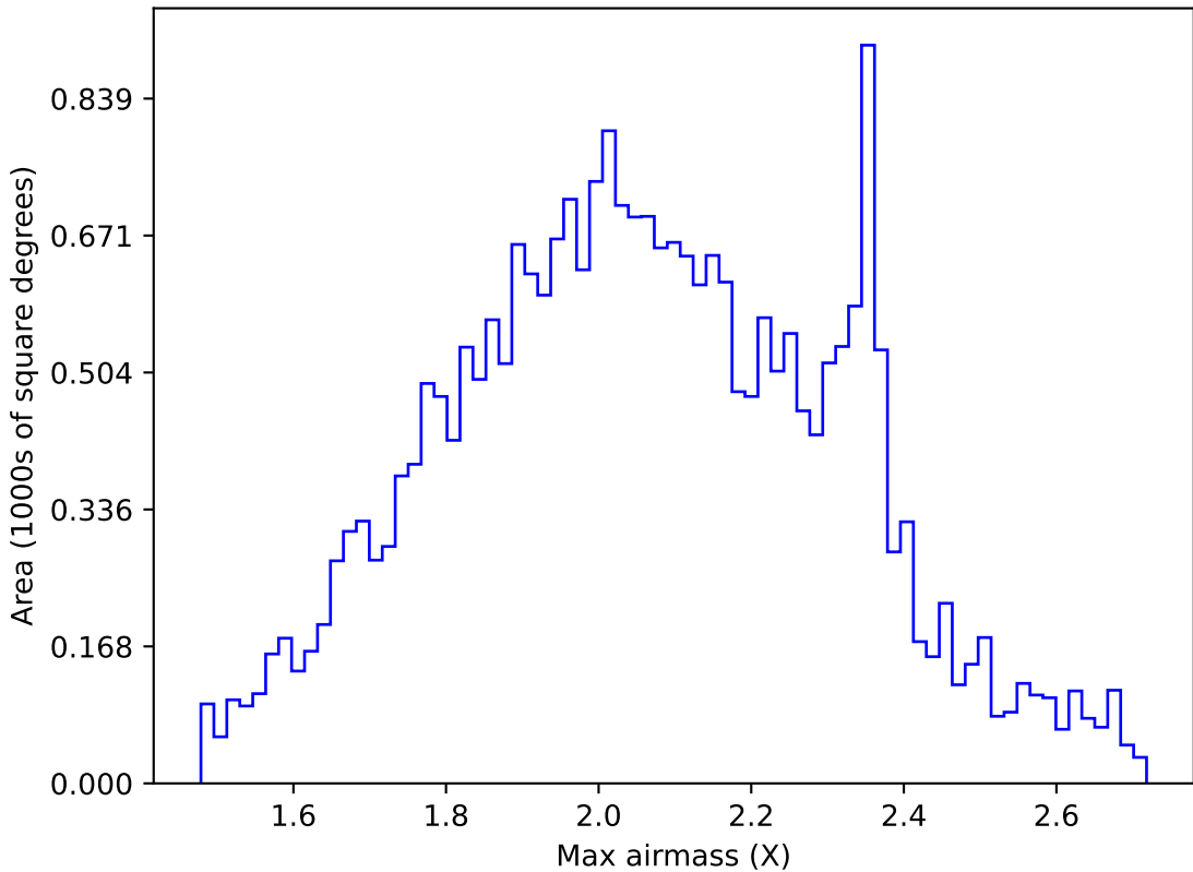
too_elab_r32_d3_griz_v3.4_10yrs All sky g band: Max airmass
