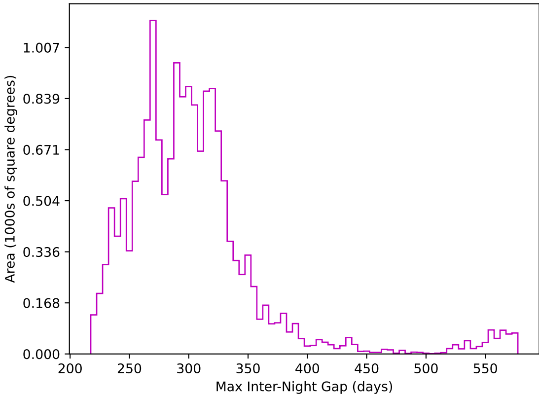
too_elab_r32_d3_griz_v3.4_10yrs WFD z band: Max Inter-Night Gap
