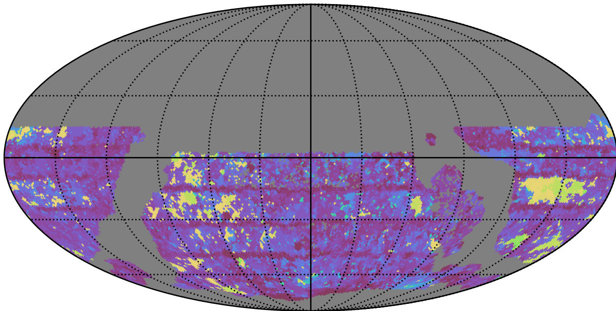
too_elab_r32_d3_griz_v3.4_10yrs WFD y band: Max Inter-Night Gap
