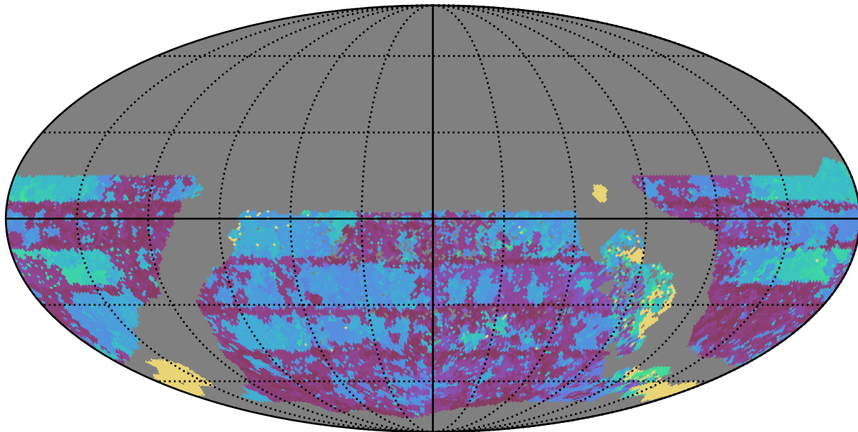
too_elab_r32_d3_griz_v3.4_10yrs WFD u band: Max Inter-Night Gap
