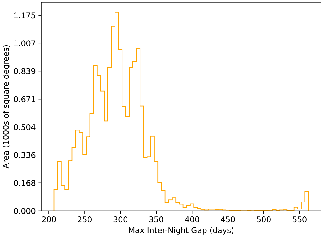
too_elab_r32_d3_griz_v3.4_10yrs WFD r band: Max Inter-Night Gap
