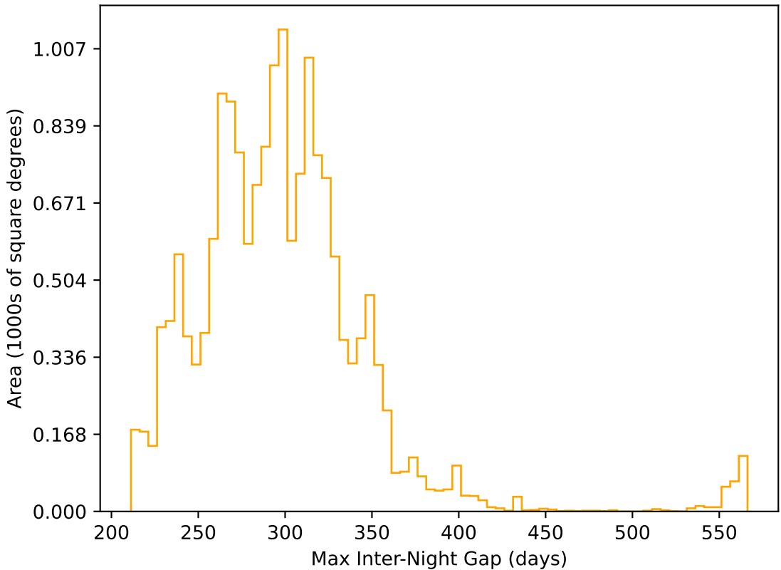
too_elab_r32_d3_griz_v3.4_10yrs WFD r band: Max Inter-Night Gap
