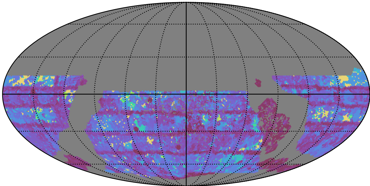
too_elab_r32_d3_griz_v3.4_10yrs WFD i band: Max Inter-Night Gap
