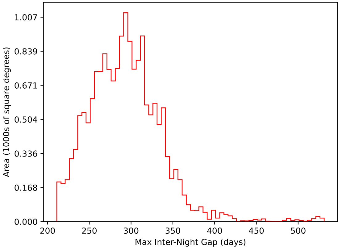
too_elab_r32_d3_griz_v3.4_10yrs WFD i band: Max Inter-Night Gap
