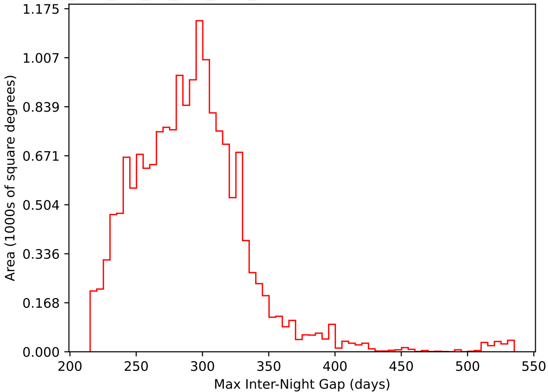
too_elab_r32_d3_griz_v3.4_10yrs WFD i band: Max Inter-Night Gap
