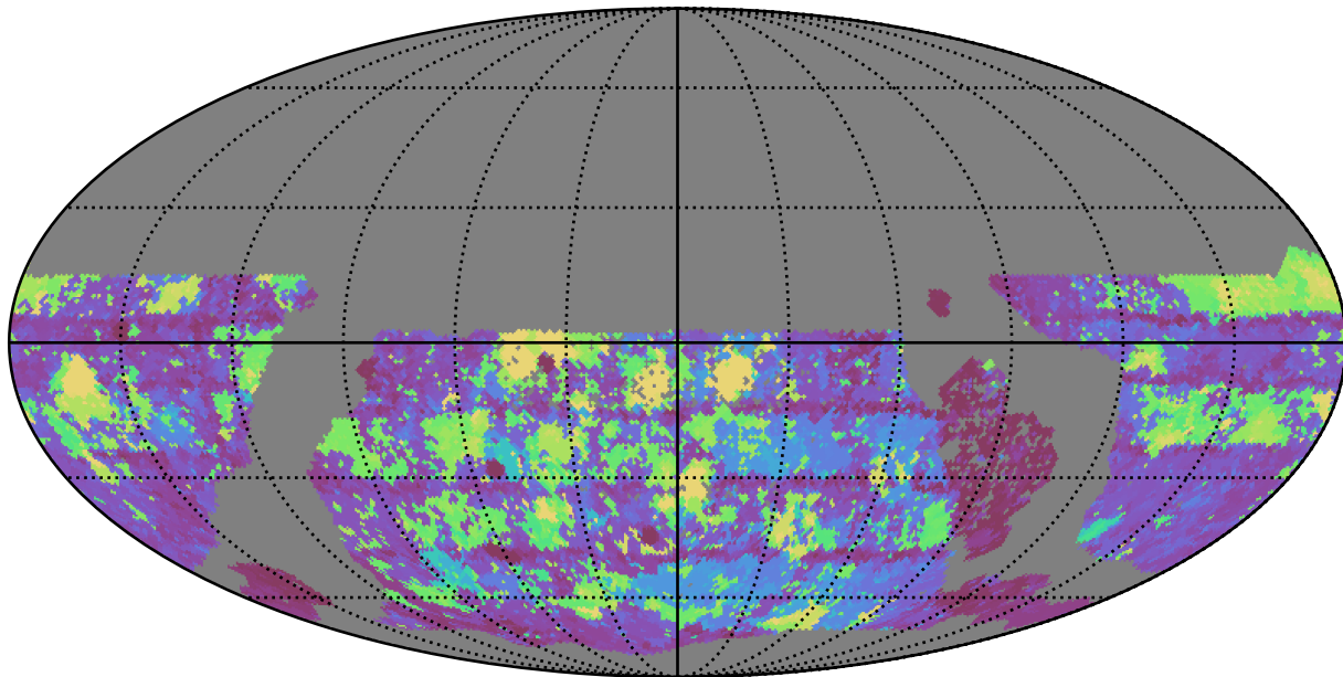
too_elab_r32_d3_griz_v3.4_10yrs WFD g band: Max Inter-Night Gap
