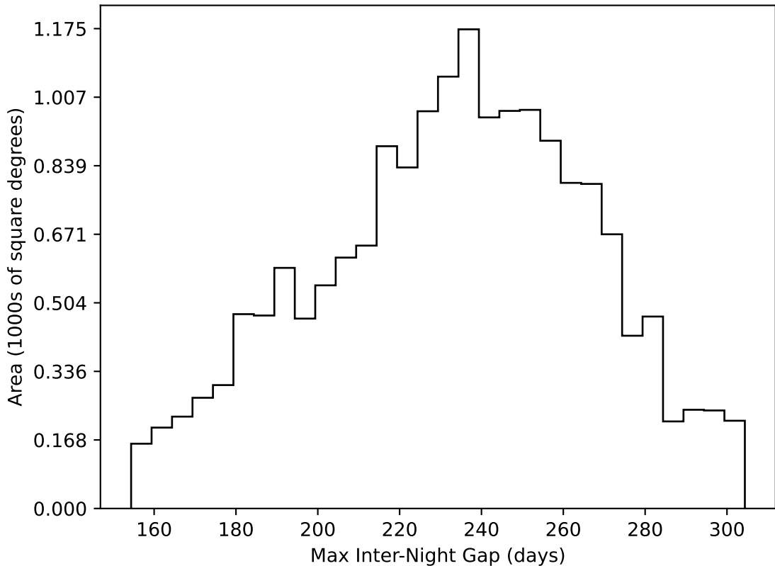
too_elab_r32_d3_griz_v3.4_10yrs WFD all bands: Max Inter-Night Gap
