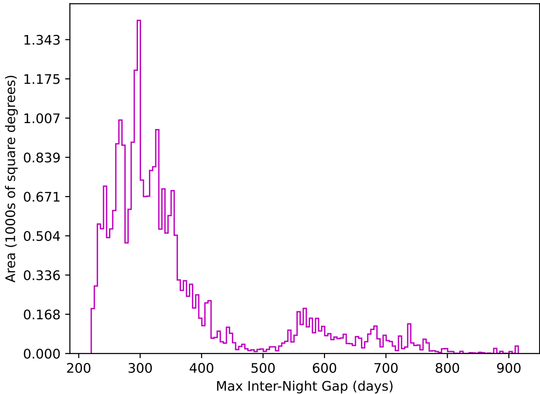
too_elab_r32_d3_griz_v3.4_10yrs All sky z band: Max Inter-Night Gap
