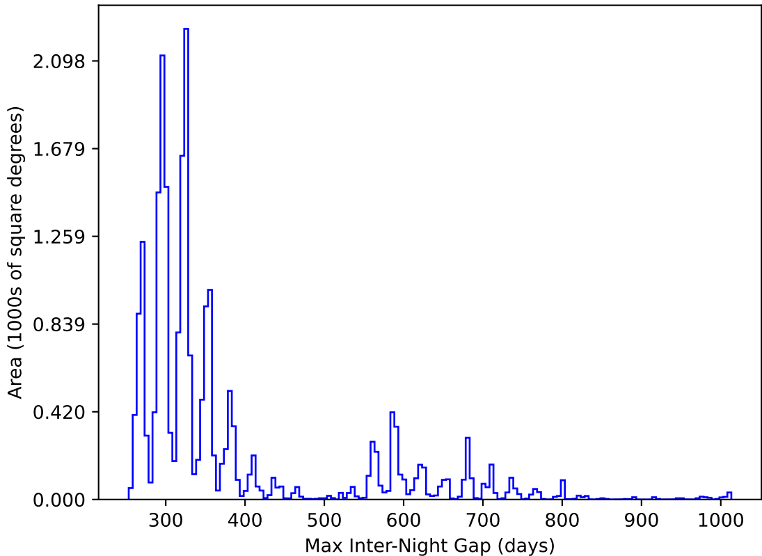
too_elab_r32_d3_griz_v3.4_10yrs All sky y band: Max Inter-Night Gap
