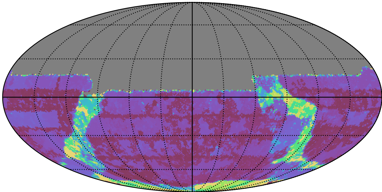
too_elab_r32_d3_griz_v3.4_10yrs All sky u band: Max Inter-Night Gap
