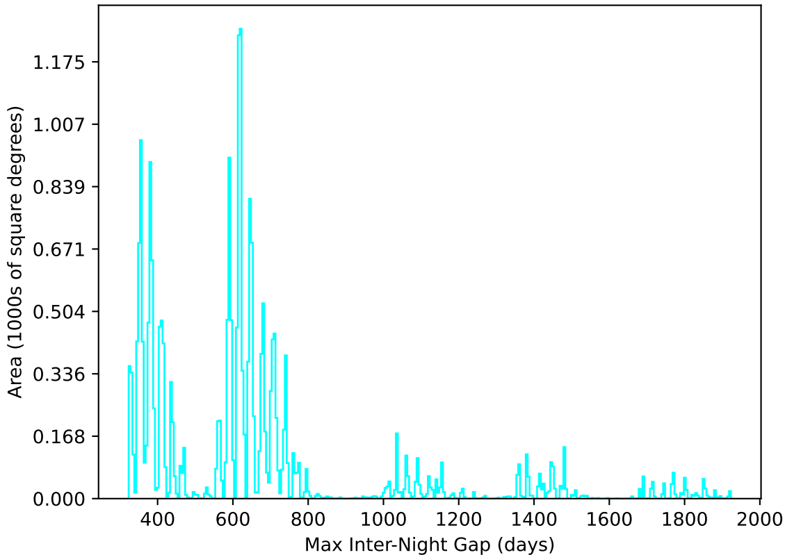
too_elab_r32_d3_griz_v3.4_10yrs All sky u band: Max Inter-Night Gap
