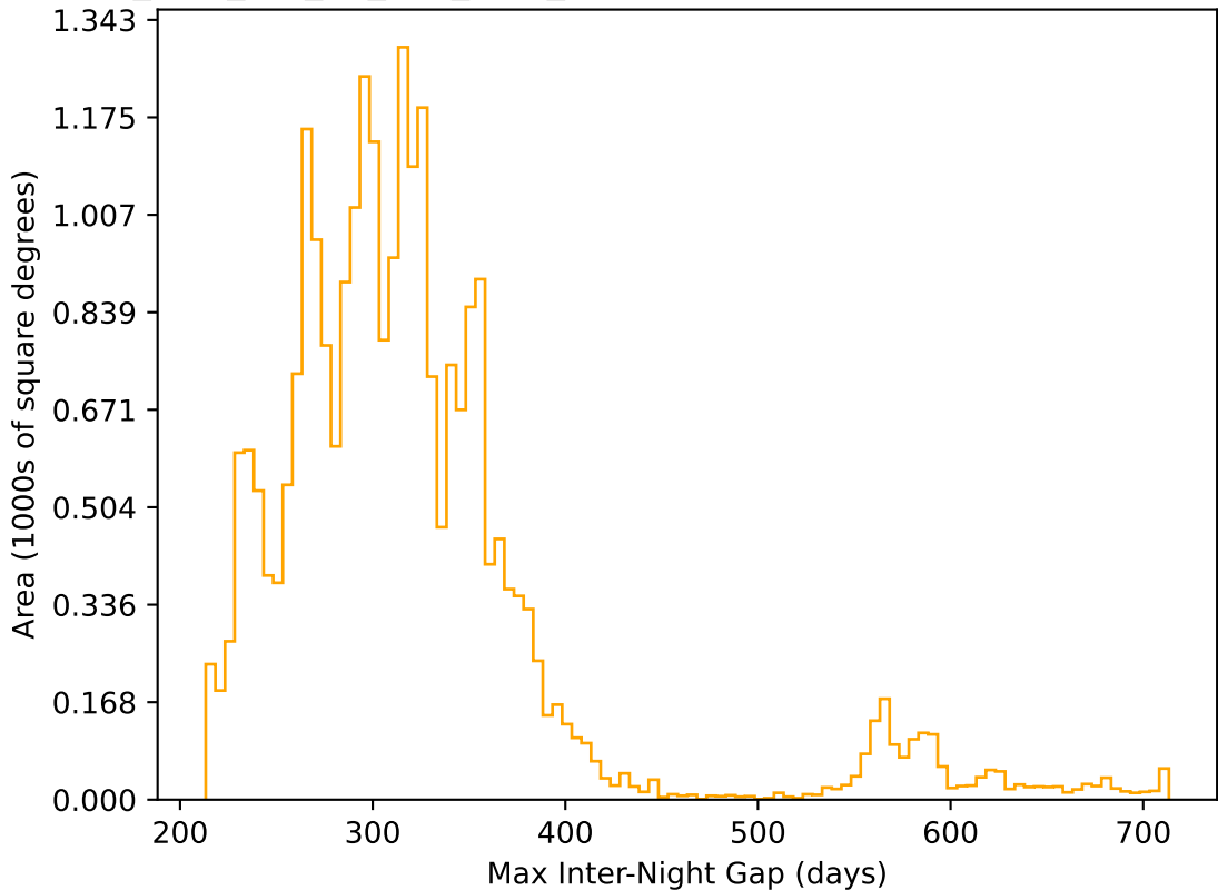
too_elab_r32_d3_griz_v3.4_10yrs All sky r band: Max Inter-Night Gap
