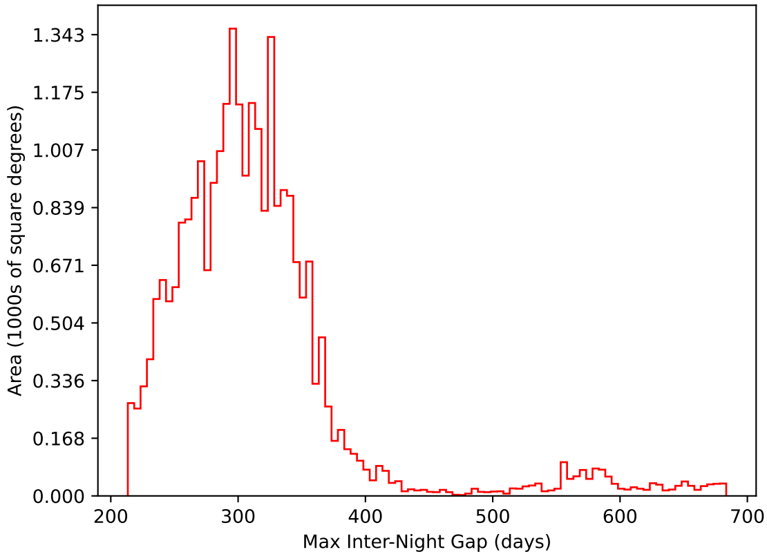
too_elab_r32_d3_griz_v3.4_10yrs All sky i band: Max Inter-Night Gap
