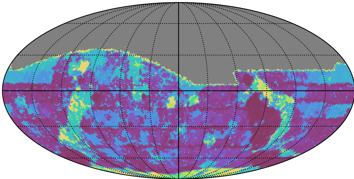
too_elab_r32_d3_griz_v3.4_10yrs All sky g band: Max Inter-Night Gap
