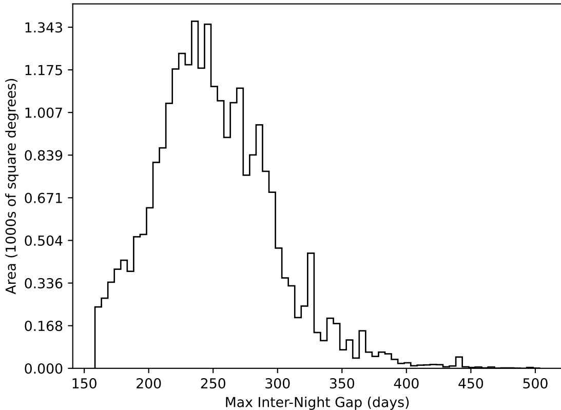
too_elab_r32_d3_griz_v3.4_10yrs All sky all bands: Max Inter-Night Gap
