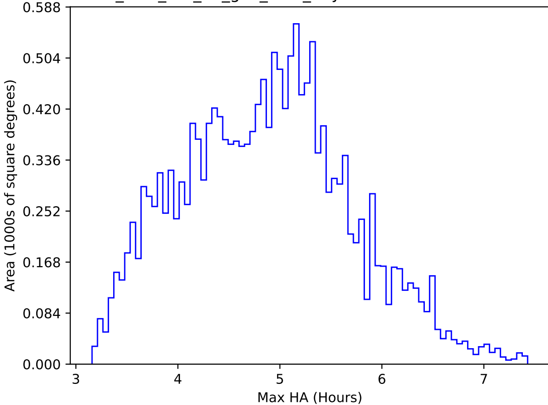
too_elab_r32_d3_griz_v3.4_10yrs WFD z band: Max HA
