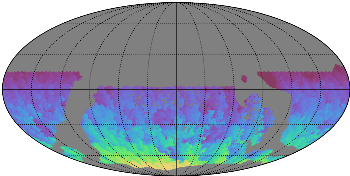
too_elab_r32_d3_griz_v3.4_10yrs WFD y band: Max HA
