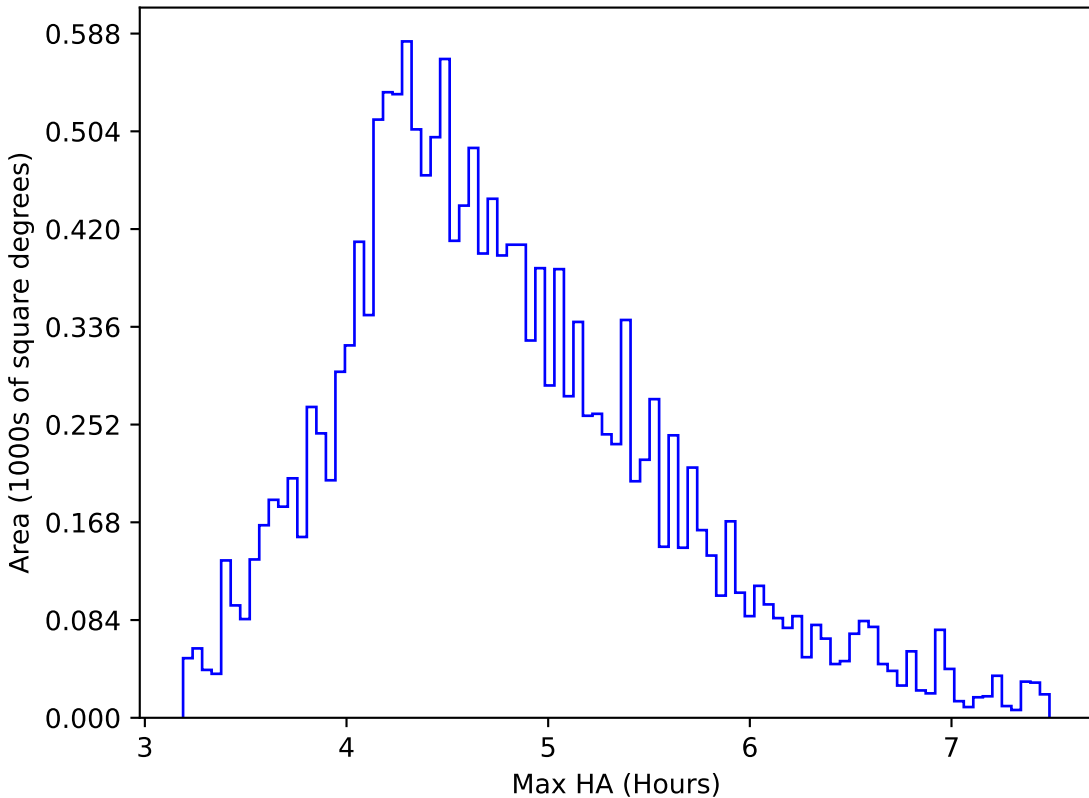
too_elab_r32_d3_griz_v3.4_10yrs WFD y band: Max HA
