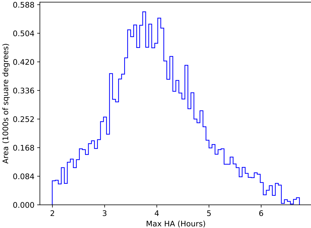
too_elab_r32_d3_griz_v3.4_10yrs WFD u band: Max HA
