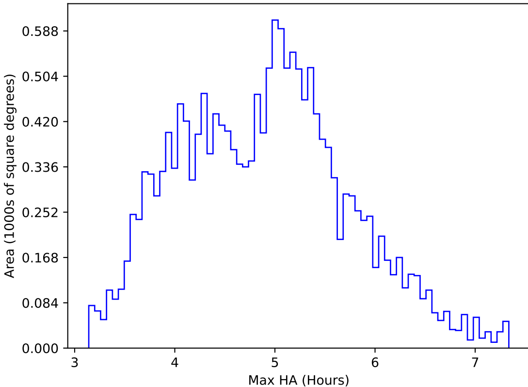
too_elab_r32_d3_griz_v3.4_10yrs WFD i band: Max HA
