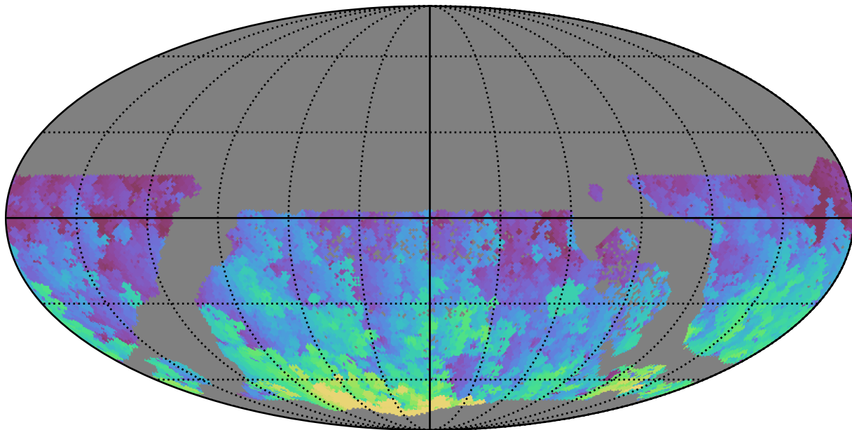
too_elab_r32_d3_griz_v3.4_10yrs WFD g band: Max HA
