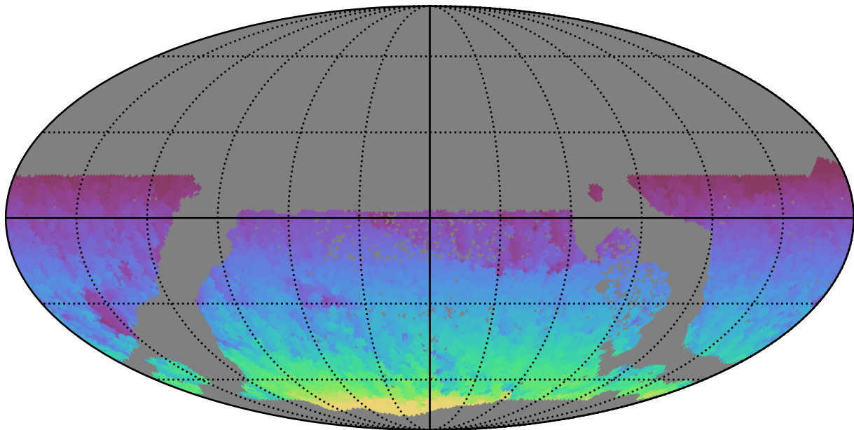
too_elab_r32_d3_griz_v3.4_10yrs WFD all bands: Max HA
