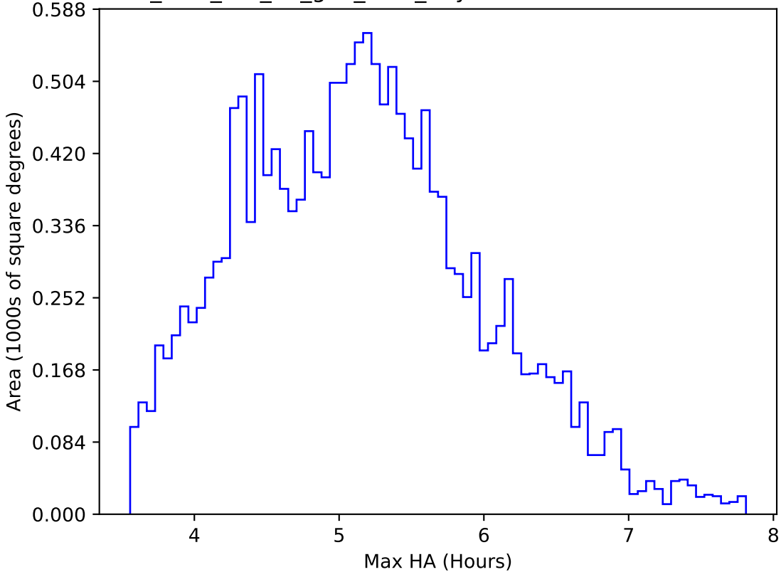
too_elab_r32_d3_griz_v3.4_10yrs WFD all bands: Max HA
