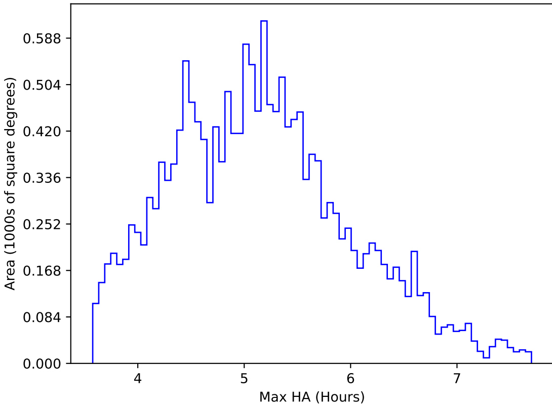
too_elab_r32_d3_griz_v3.4_10yrs WFD all bands: Max HA
