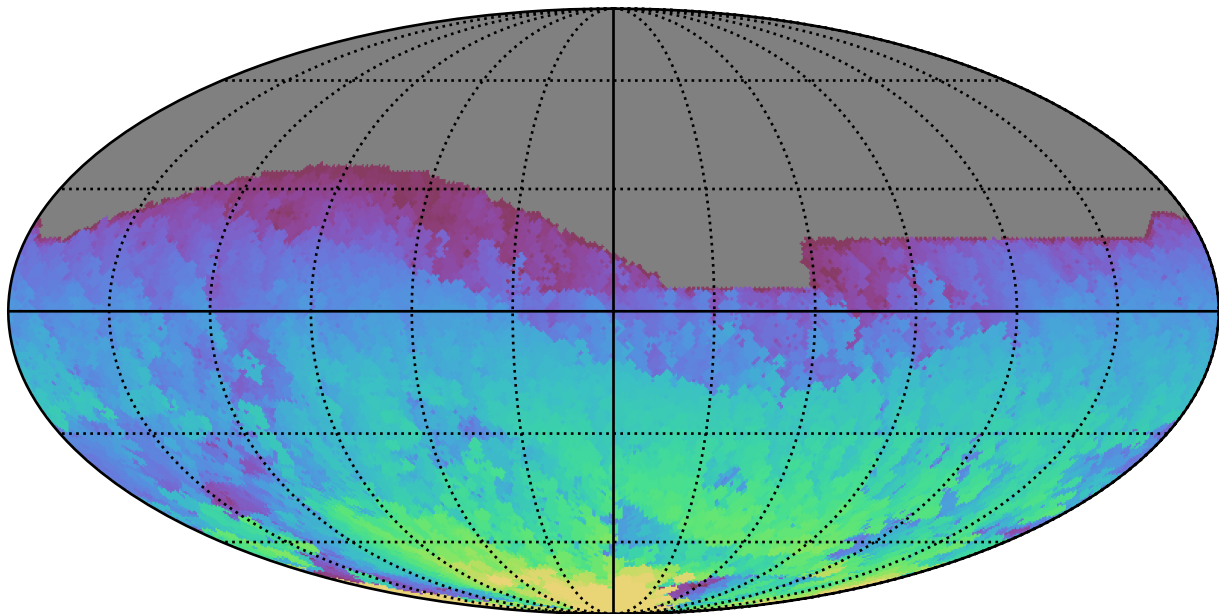
too_elab_r32_d3_griz_v3.4_10yrs All sky z band: Max HA
