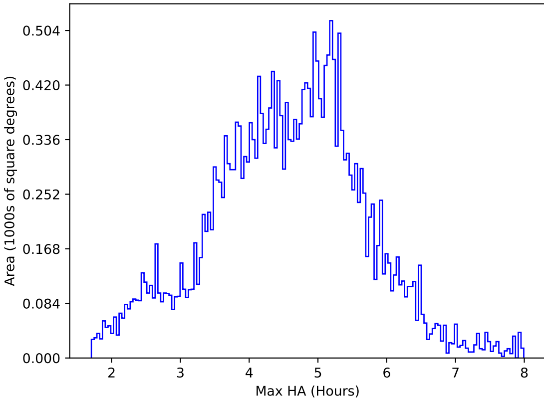
too_elab_r32_d3_griz_v3.4_10yrs All sky z band: Max HA
