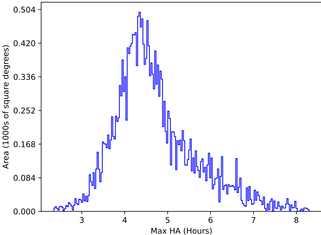
too_elab_r32_d3_griz_v3.4_10yrs All sky y band: Max HA
