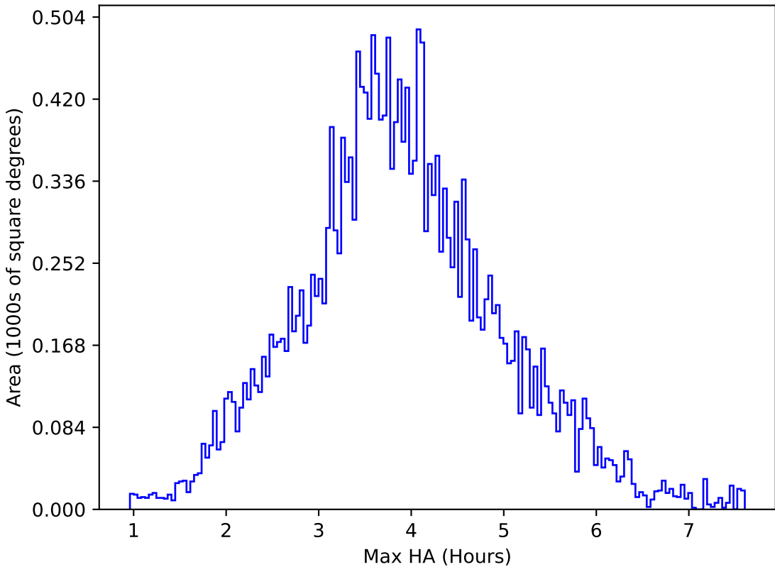
too_elab_r32_d3_griz_v3.4_10yrs All sky u band: Max HA
