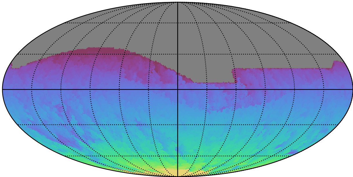
too_elab_r32_d3_griz_v3.4_10yrs All sky all bands: Max HA
