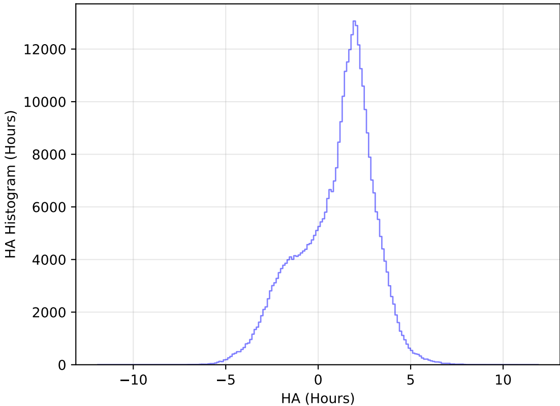
too_elab_r32_d3_griz_v3.4_10yrs WFD y band: HA Histogram
