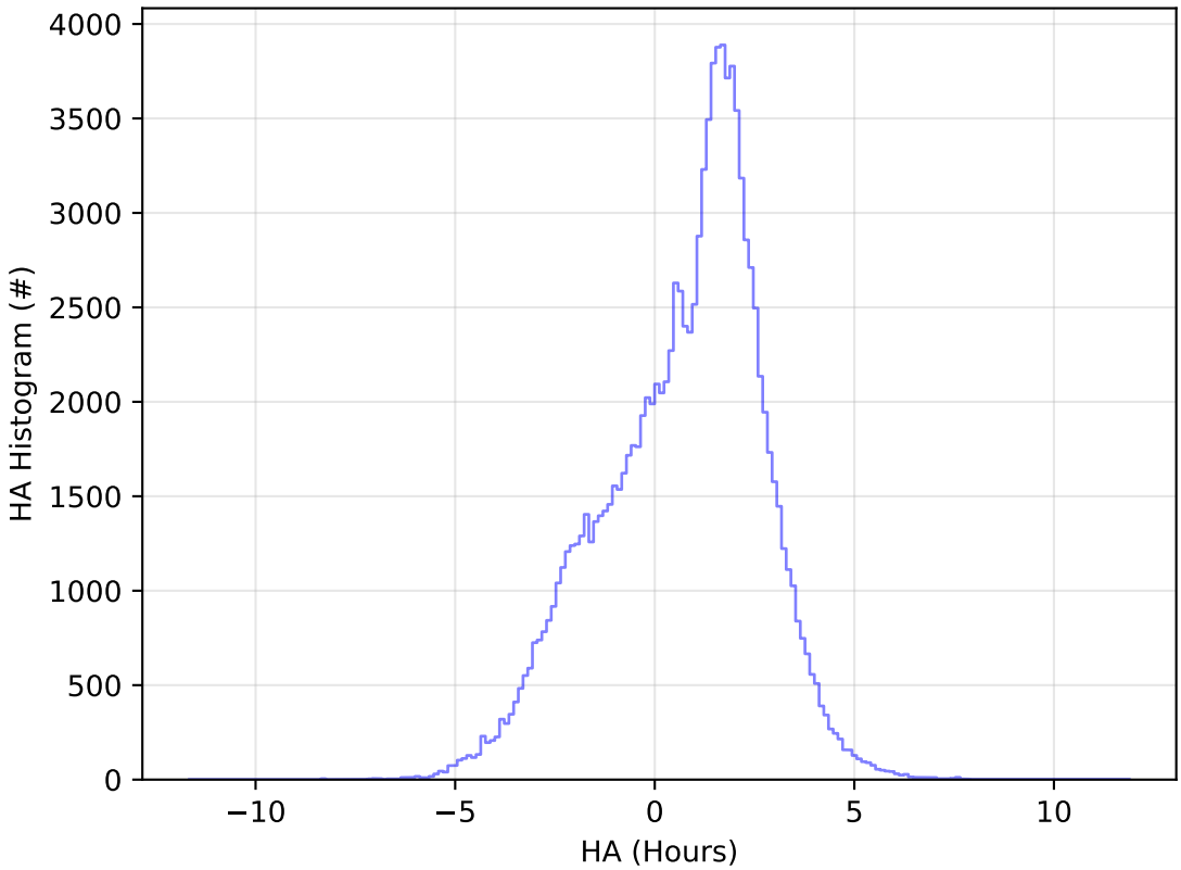
too_elab_r32_d3_griz_v3.4_10yrs WFD u band: HA Histogram
