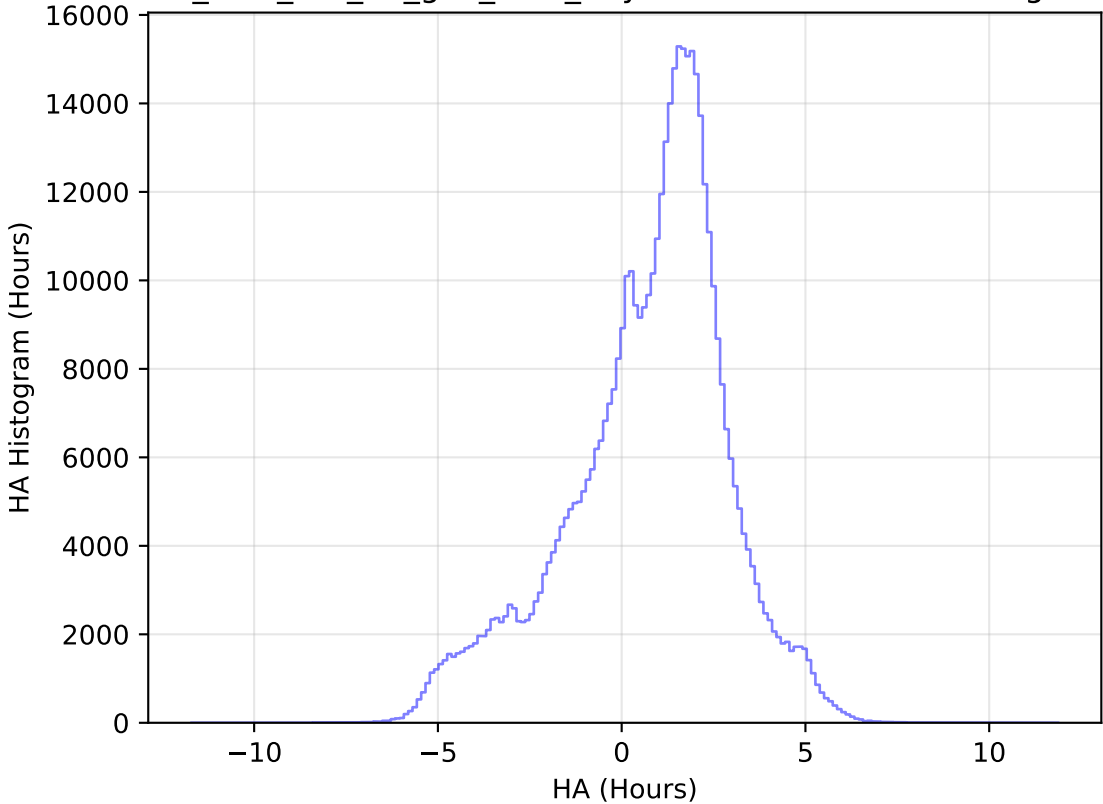
too_elab_r32_d3_griz_v3.4_10yrs WFD i band: HA Histogram
