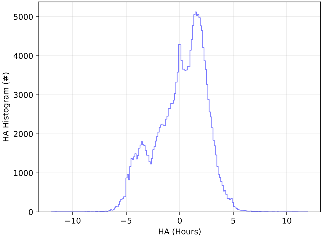
too_elab_r32_d3_griz_v3.4_10yrs WFD g band: HA Histogram
