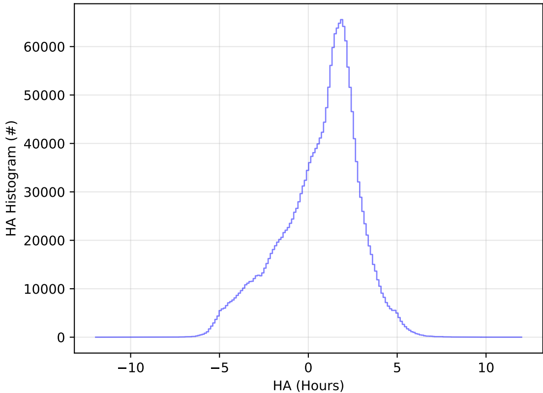
too_elab_r32_d3_griz_v3.4_10yrs WFD all bands: HA Histogram
