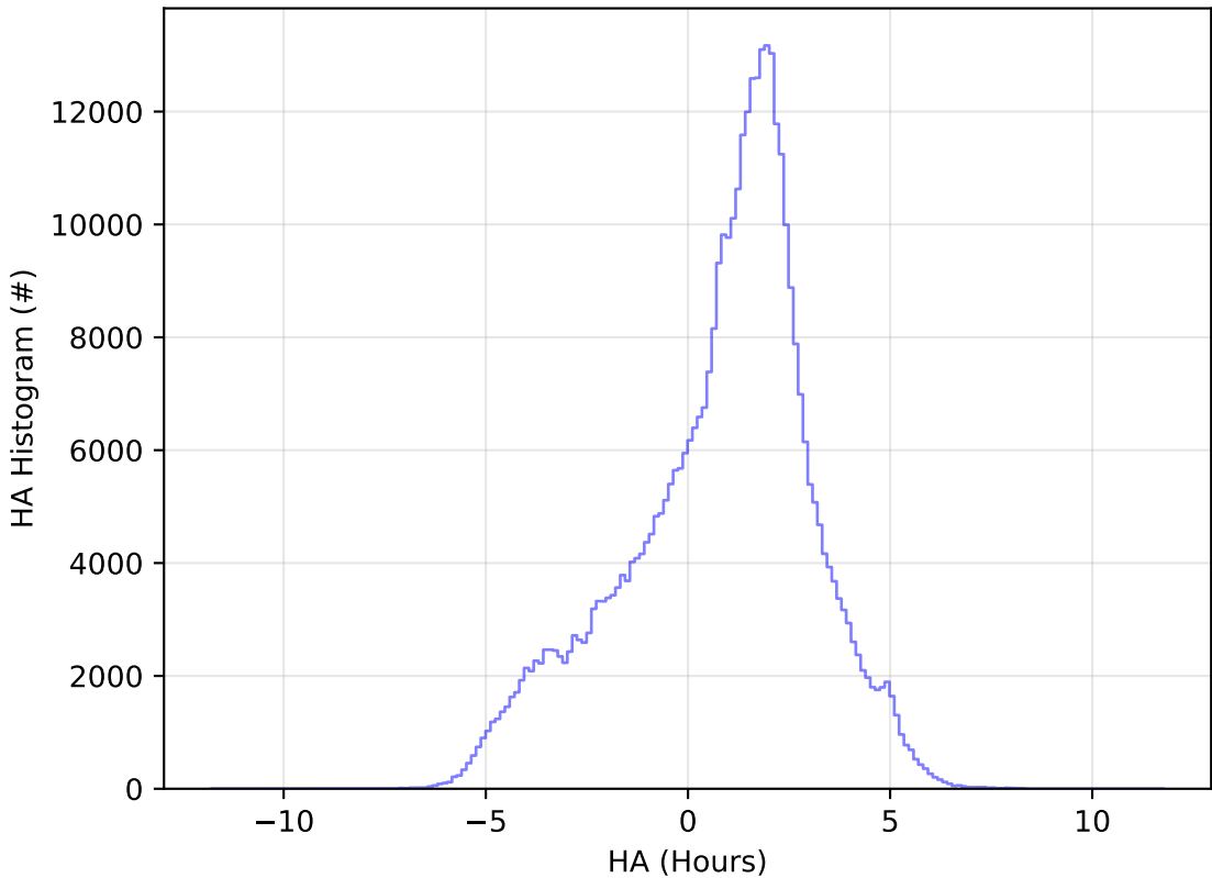
too_elab_r32_d3_griz_v3.4_10yrs All sky z band: HA Histogram
