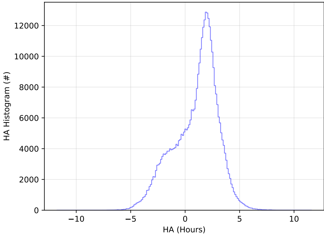
too_elab_r32_d3_griz_v3.4_10yrs All sky y band: HA Histogram
