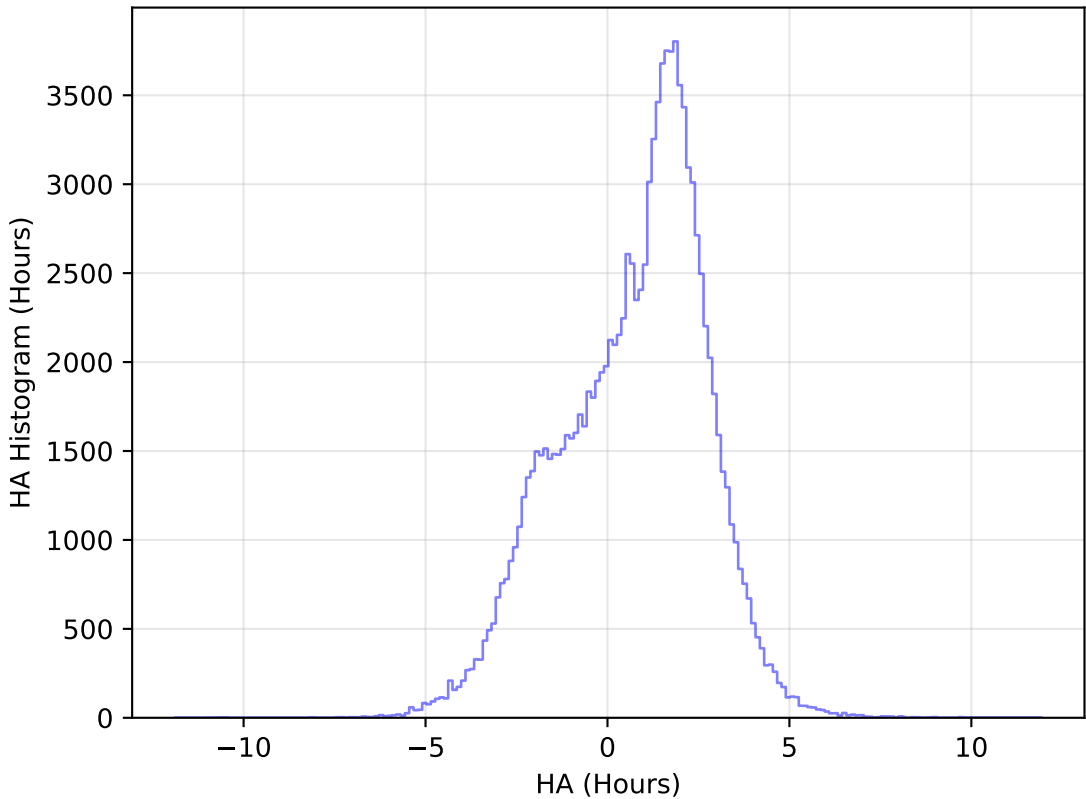
too_elab_r32_d3_griz_v3.4_10yrs All sky u band: HA Histogram
