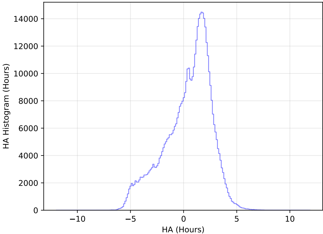
too_elab_r32_d3_griz_v3.4_10yrs All sky r band: HA Histogram
