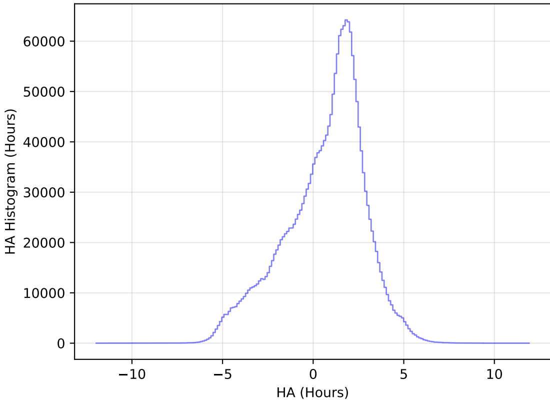
too_elab_r32_d3_griz_v3.4_10yrs All sky all bands: HA Histogram
