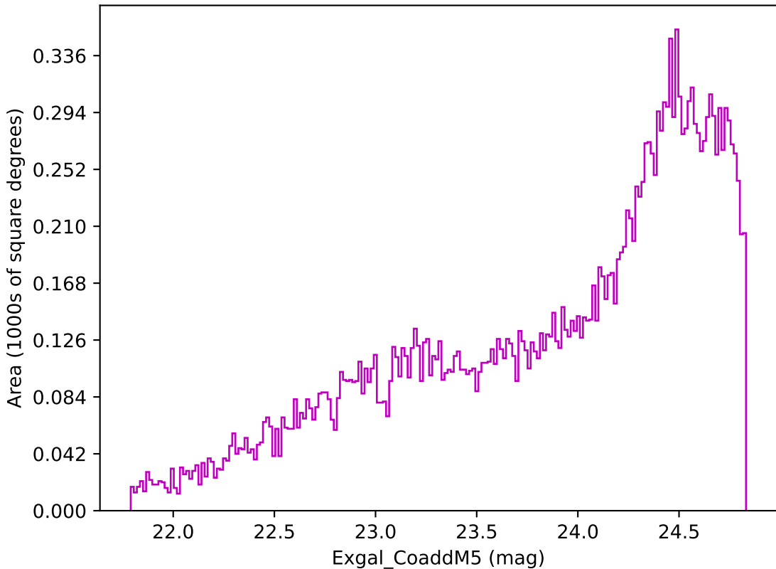
too_elab_r32_d3_griz_v3.4_10yrs Yr 3-4 z band: Exgal_CoaddM5
