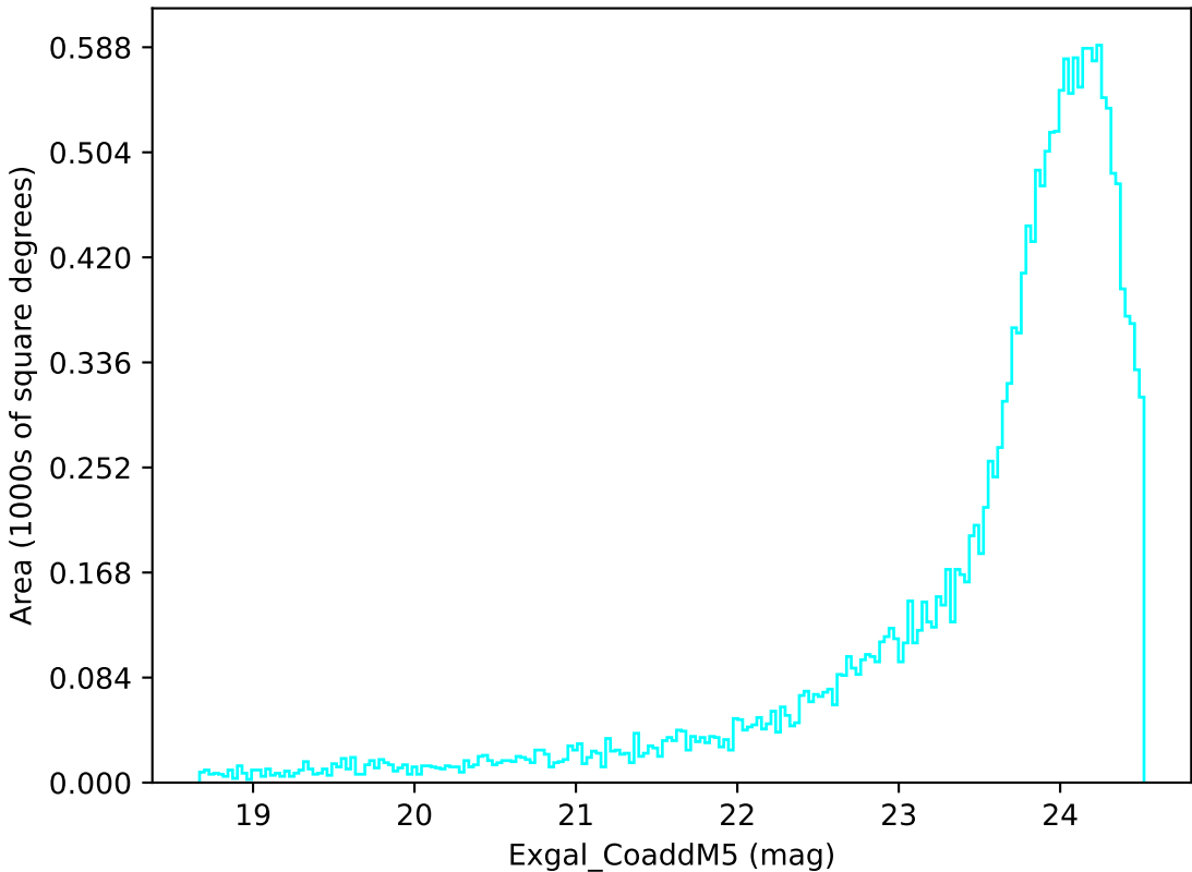
too_elab_r32_d3_griz_v3.4_10yrs Yr 1 u band: Exgal_CoaddM5
