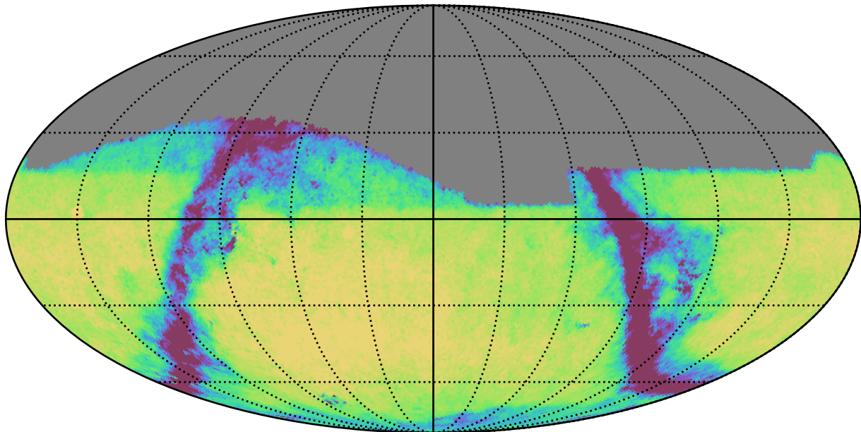
too_elab_r32_d3_griz_v3.4_10yrs Yr 1 r band: Exgal_CoaddM5
