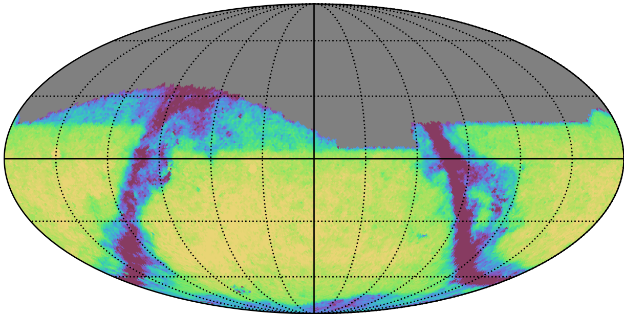
too_elab_r32_d3_griz_v3.4_10yrs Yr 1 i band: Exgal_CoaddM5
