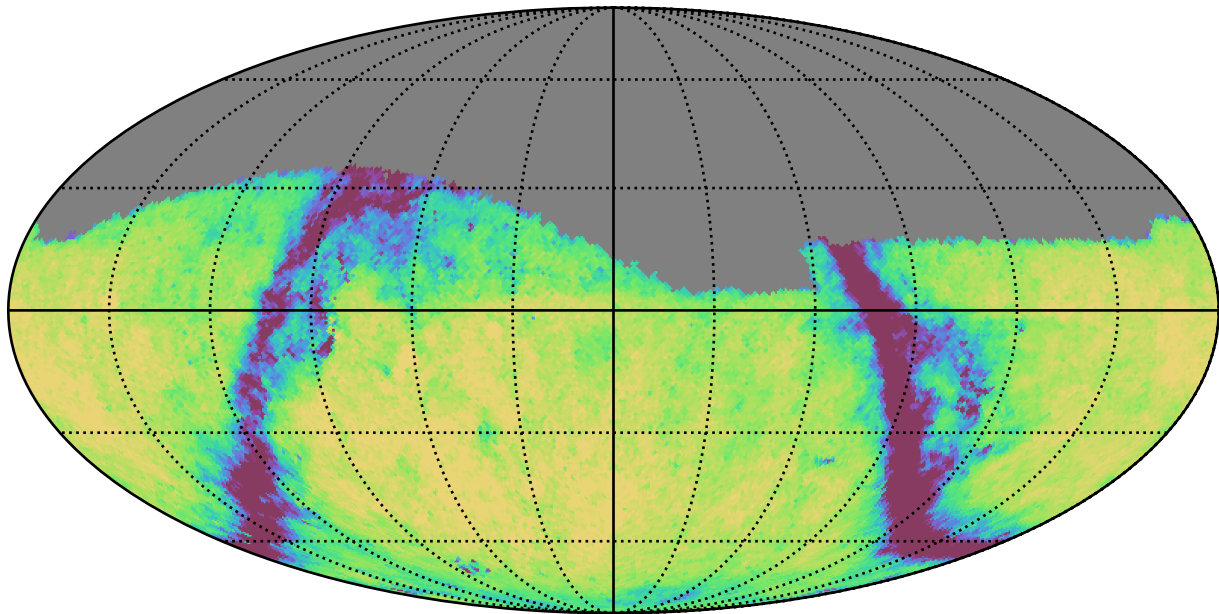
too_elab_r32_d3_griz_v3.4_10yrs Yr 1 g band: Exgal_CoaddM5
